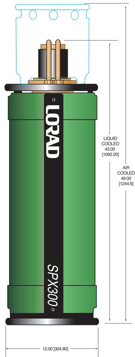
SPX300 TUBE HEAD SIDE VIEW
