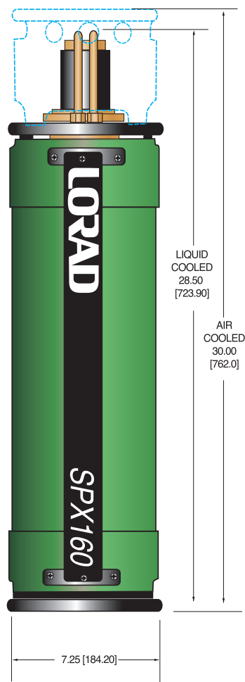
SPX160 TUBE HEAD SIDE VIEW
